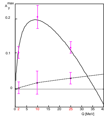
Fig. 2: Error bars of the analysing power amplitude as expected from the planned measurement [8]. The solid line depicts predictions of A_y^{\text{max}} according to [1]. The dashed line connects the predictions of the model from reference [2] as calculated for Q = 2, 10, 25, and 40 MeV [9]. The dashed line is plotted to guide the eye. In case of the model from reference [2] the A_y^{\text{max}} is not well defined and in the figure we show an average of the modulus from maximum negative and positive value of A_y .
