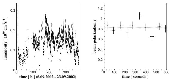
Fig. 1: (a) On-line determination of the luminosity during the September '02 measurements of \bar{p}p \rightarrow pp\eta reaction. (b) On-line estimation of the beam polarization as measured using the EDDA polarimeter – the value of vertical beam polarization is shown versus the time of the cycle.
